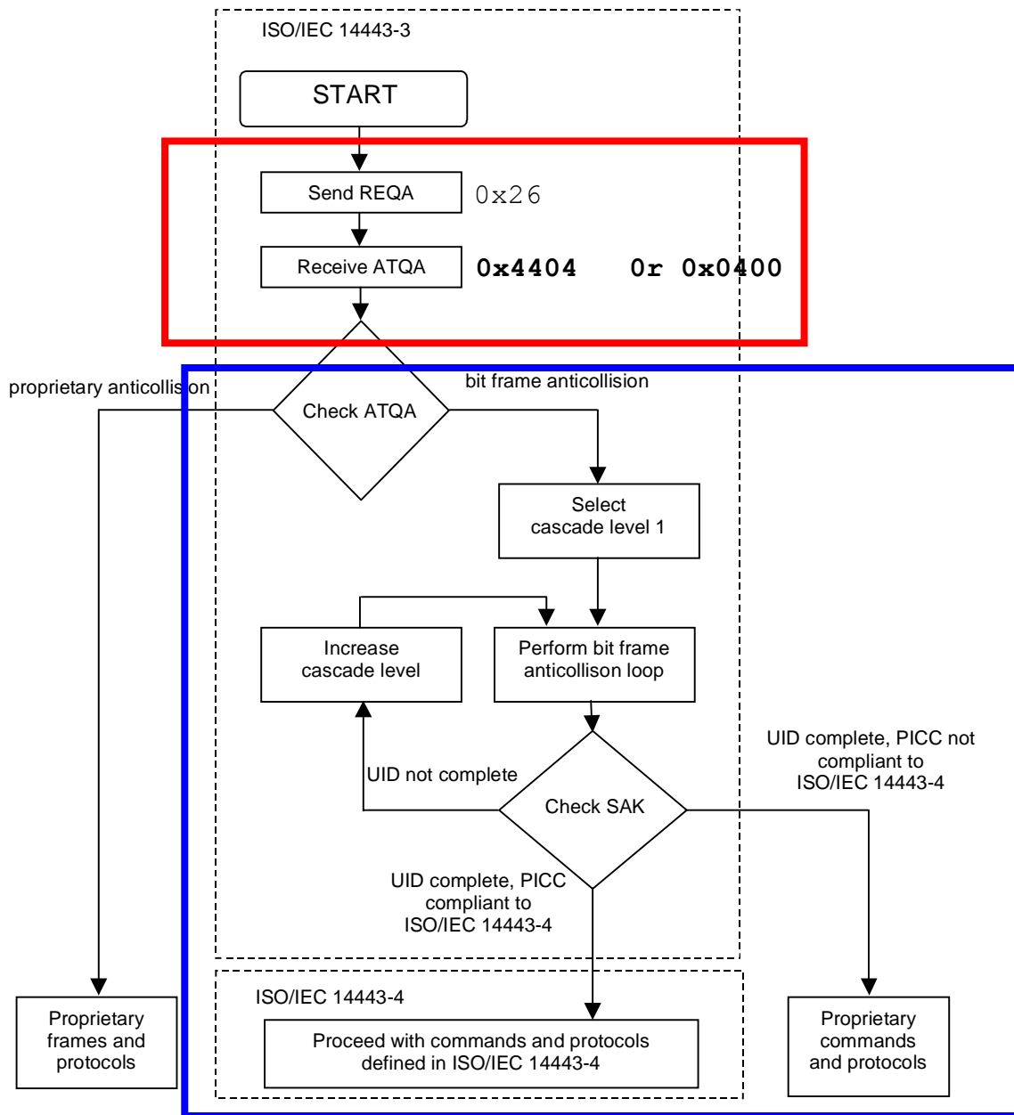
Figure 8 — Initialization and anticollision flowchart for PCD
