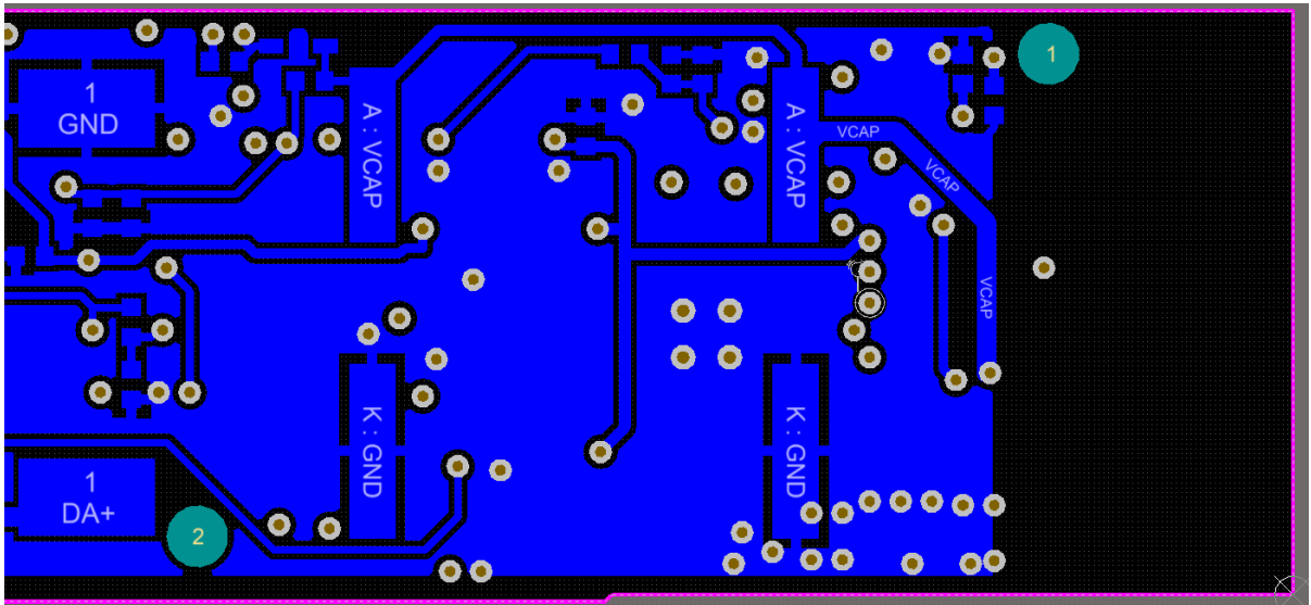
Layer 4 (bottom)
