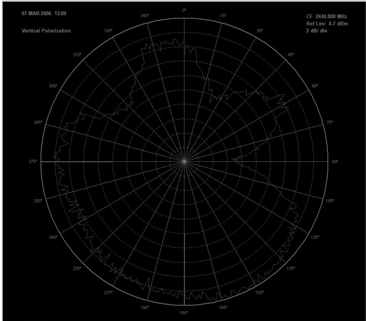
Figure 1 Radiation plot - nRF24L01-REFMOD - Vertical Polarization – Ref. level = -1.9dBm
