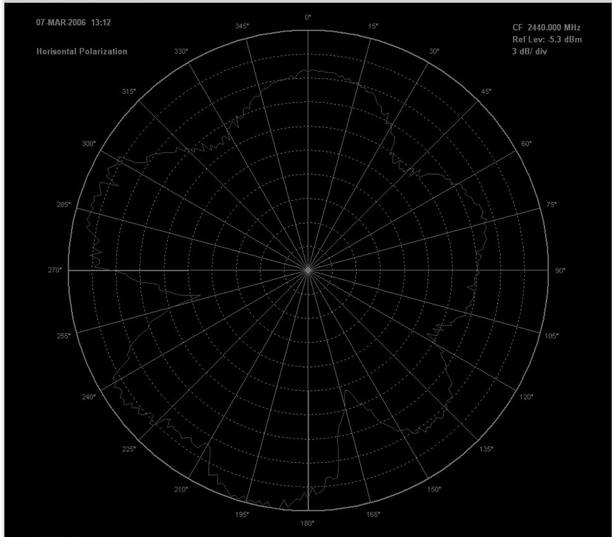
Figure 2 plot - nRF24L01-REFMOD - Horizontal Polarization – Ref. level = -1.1dBm
