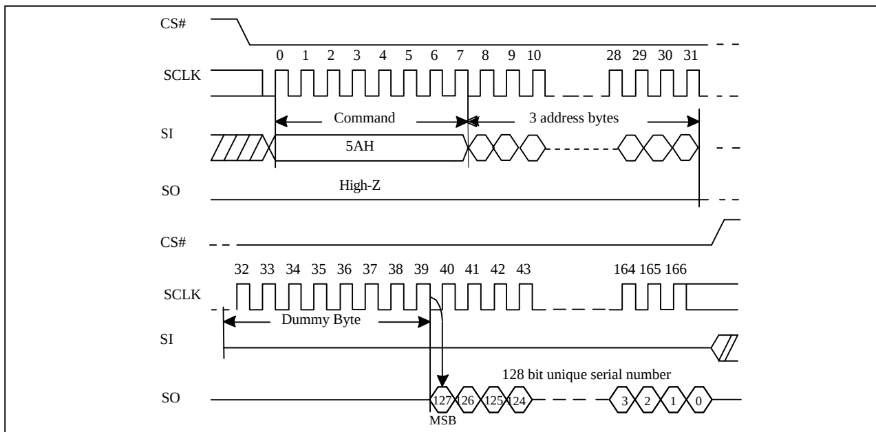
Figure 37.1. Read Unique ID (RUID) Sequence (Command 5AH)
