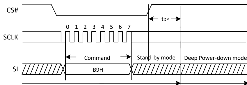
Figure 24. Deep Power-Down Sequence Diagram
