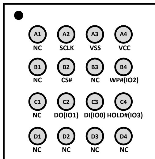
16-ball TFBGA
