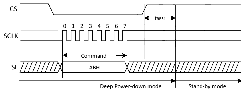
Figure 26. Release Power-Down/Read Device ID Sequence Diagram
