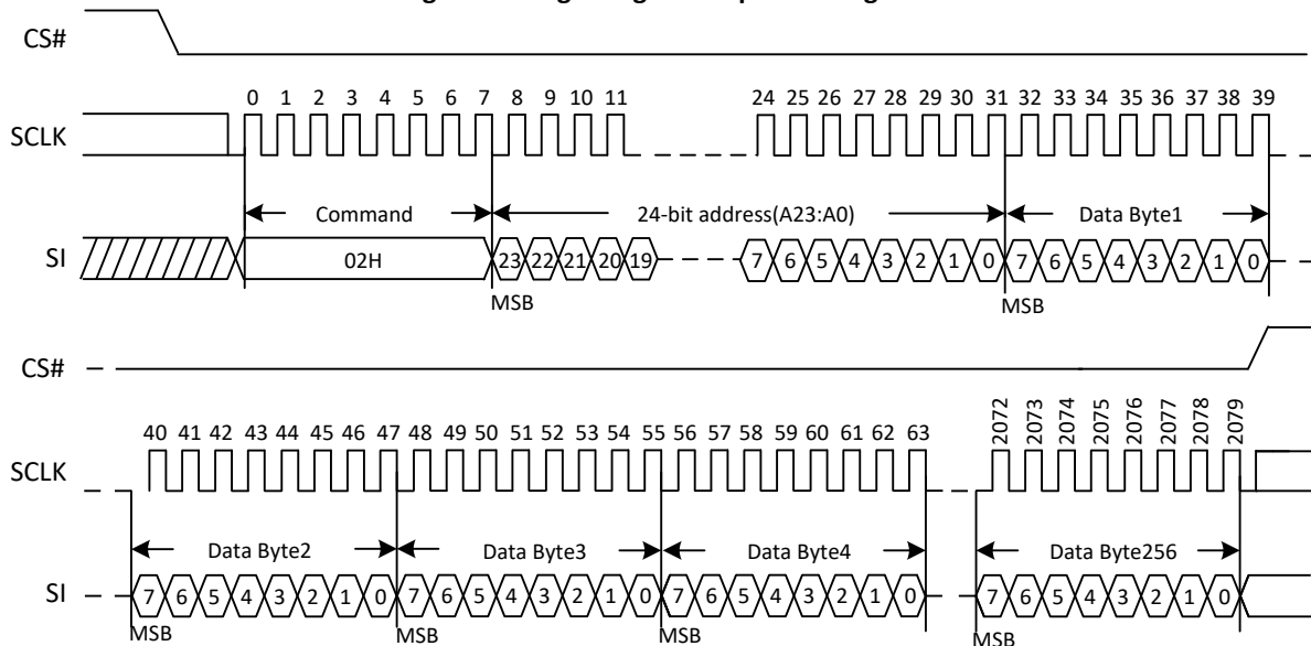
Figure 17. Page Program Sequence Diagram
