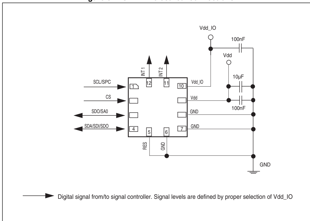
Figure 5. LIS2DH12 electrical connections
