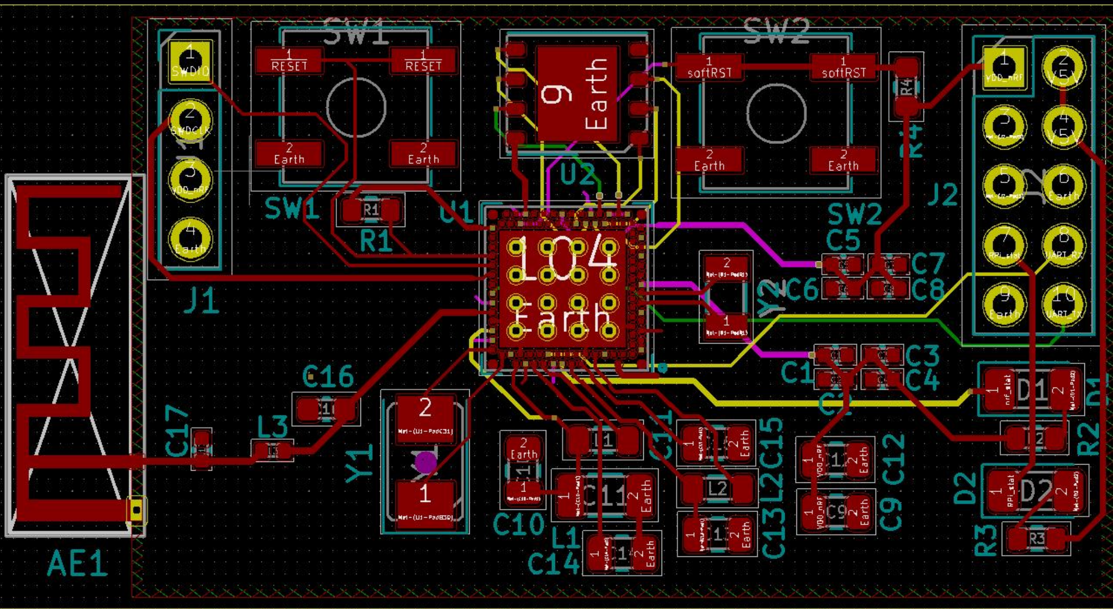
PCB Layout
