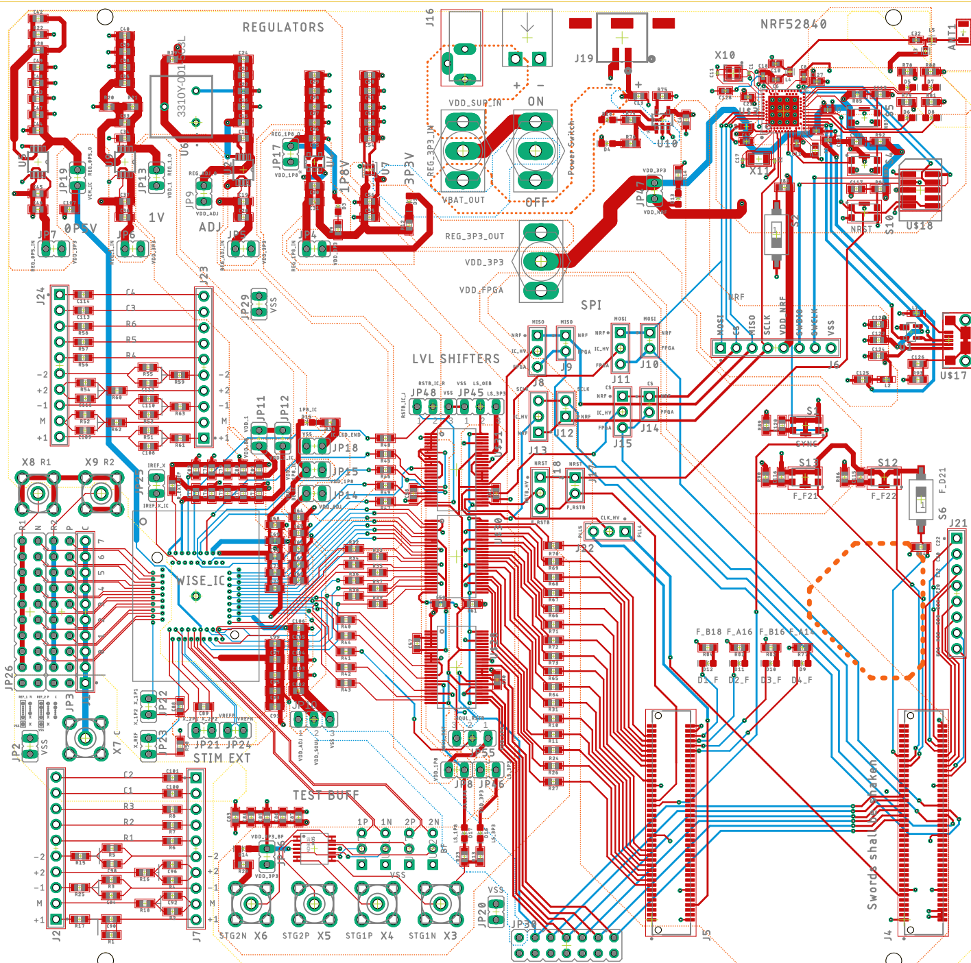
Ear EEG Bring Up Board Justin Doong, Sina Faraji, Ryan Kaveh
